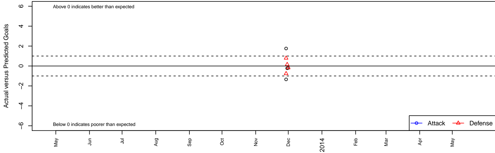
Conejo Valley United Blue G01 Dots are actual minus expected GF (blue circles) and GA (red triangles). Blue line is smoothed change in attack strength. Red is smoothed change in defense strength.
